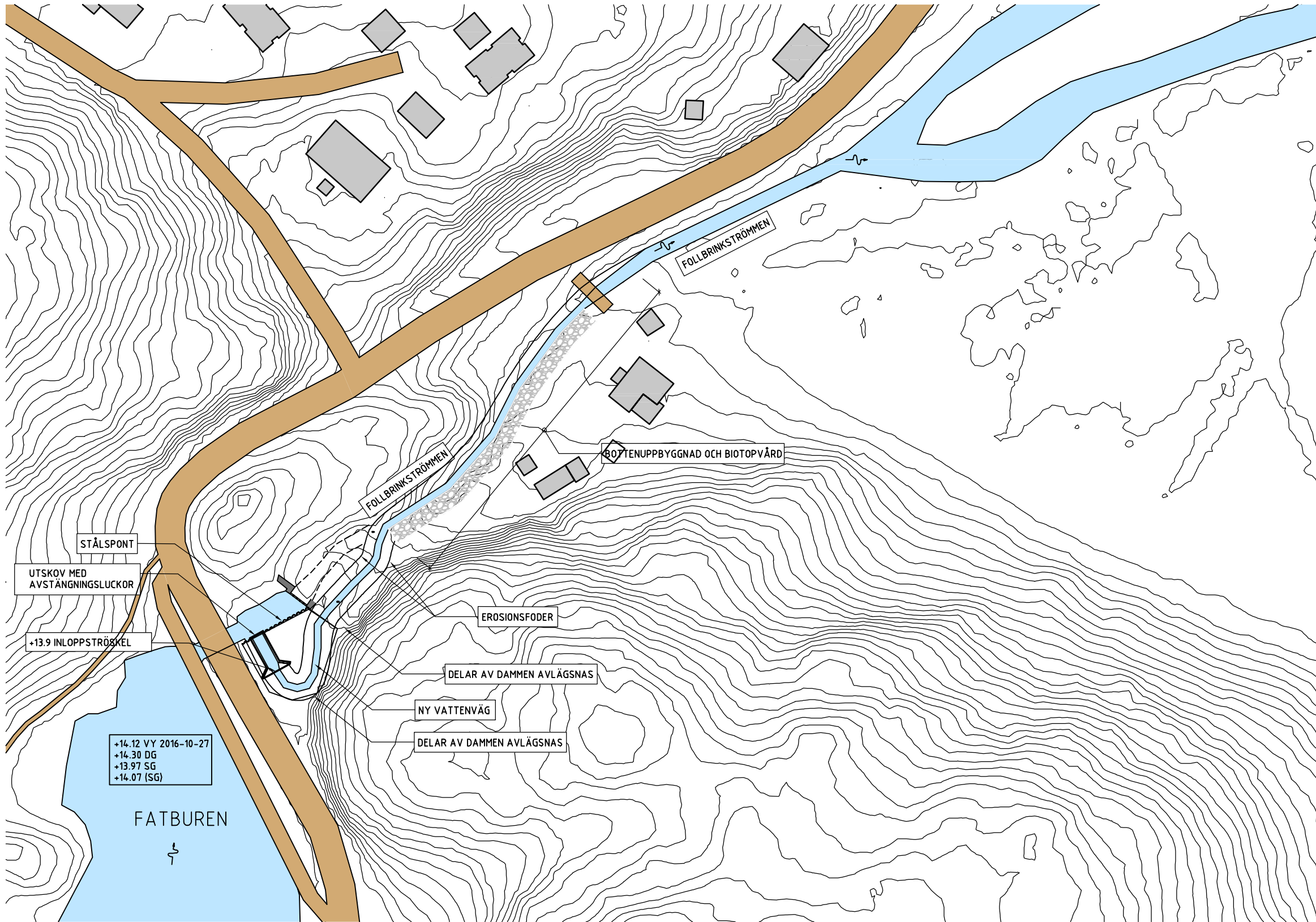
PLAN SKALA 1:500
